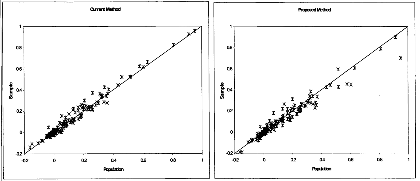
Figure 2. Pairwise product moment correlations for 20 variables after subsampling and microaggregation
