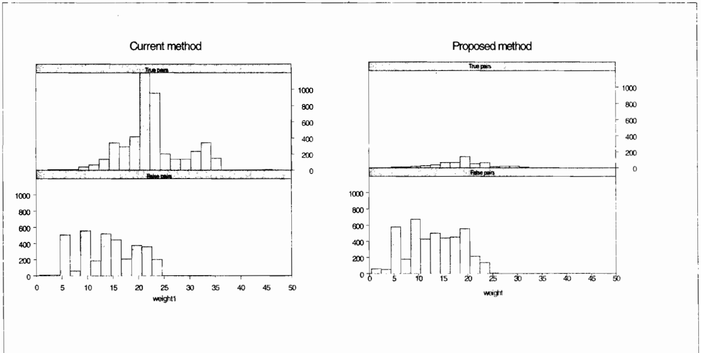
Figure 1. Histogram of match weights for true and false match pairs
